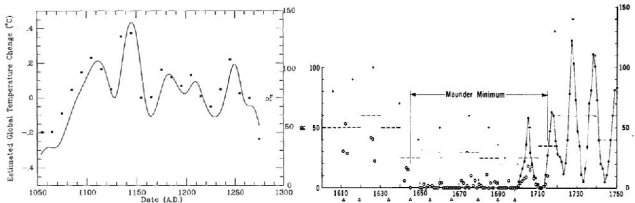
Figure 1.18. (Left) \Delta^{14}\text{C} -derived R_z (Wolf sunspot indices) estimate (solid squares) and global temperature model predictions (curve) (after Jirikowic and Damon, 1994). (Right) Estimated annual mean sunspot numbers from 1610 to 1750; dashed lines are decade's estimates, crosses are peak estimates and triangles are Wolf's estimated dates of maxima for an assumed 11.1-year solar cycle (after Eddy, 1976).
