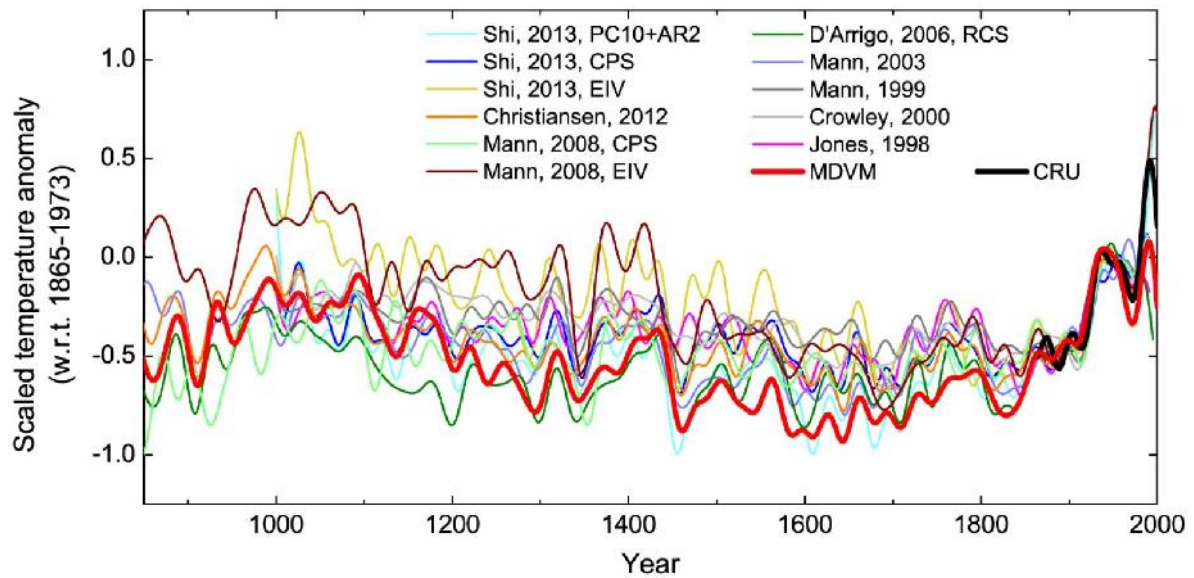
Figure 1.17. Several reconstructions for the mean temperature of the Northern Hemisphere. All reconstructions were 30-year low-pass filtered, and scaled to the smoothed instrumental series by the variance and mean over the common period AD 1865–1973 (more details in Xing et al., 2016, from which this Figure was reproduced).
