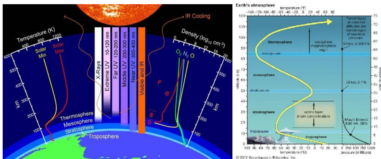
Figure 1.11. (Left) Layers of the Earth's atmosphere (troposphere, stratosphere, mesosphere and thermosphere), showing the temperature difference with increasing altitude from Earth for both solar minimum and solar maximum periods, the atmospheric penetration of the various spectral wavelengths, the density of some chemical species with increasing altitude from the Earth, and the approximate height within the D, E and F levels of the ionosphere (credit: John Emmert/NRL, NASA) https://science.nasa.gov/science-news/science-at-nasa/2010/15jul_thermosphere . (Right) Graphic showing also the ionosphere, overlapping the mesosphere and thermosphere; parts of the ionosphere overlap with magnetosphere, shaped by the solar wind's interaction with the Earth's magnetic field. The yellow line shows the response of air temperature to increasing height (credit: Encyclopædia Britannica, Inc.).
