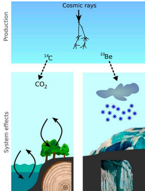
Figure 1.10. Picture showing some fundamentals of the radioisotopes ^{14}\text{C} and ^{10}\text{Be} in the Earth's system. Both are produced by nuclear reactions of GCR particles with the atmospheric gases (Masarik and Beer, 2009), but after production their fate is very different (system effects). While ^{10}\text{Be} attaches to aerosols and is transported within a few years to ground (Heikkilä et al., 2009), ^{14}\text{C} oxidizes to \text{CO}_2 and enters the global C cycle, exchanging between atmosphere, biosphere, and the oceans (Siegenthaler, 1983) (after Steinhilber et al., 2012). John Eddy (1976) was the first to recognize the strong inverse correlation between the production of the cosmogenic radionuclides and SA.
