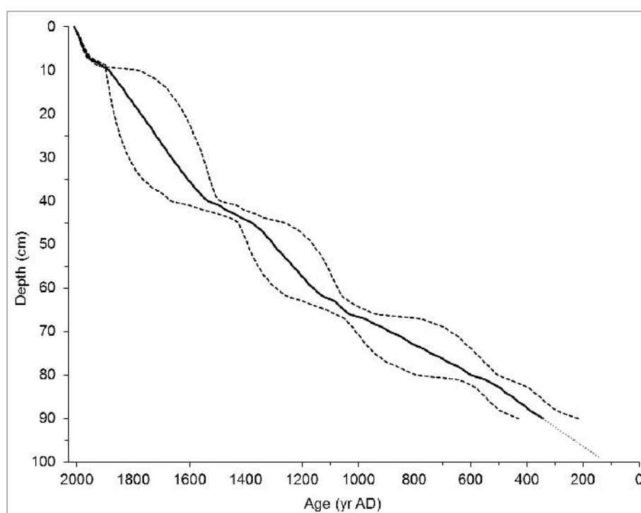
Figure 7.2. Age model for the core FCPw1 and estimated 2\sigma errors, based on six AMS- ^{14}\text{C} dates, performed on total organic sediment, and ^{210}\text{Pb} chronology. The data interpolation was obtained with Bchron 3.2 software. The lowermost 10 cm has been extrapolated from the Bchron calculation between 81 and 91 cm depth by linear regression.
